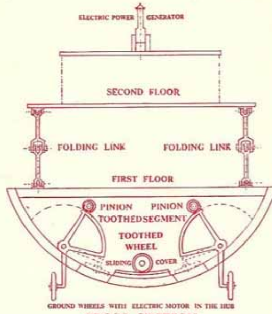
CROSS SECTION
